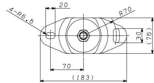
Detail of front engine mount
